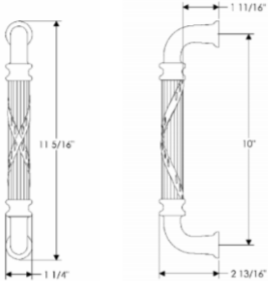
G622AP Ribbon & Reed Appliance Pull
