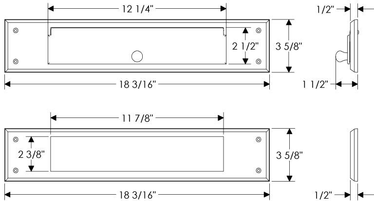
MS112 Mail Slot 18 \frac{3}{16} " x 3 \frac{5}{8} "
