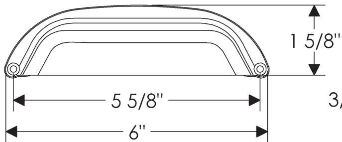
CK363 5 \frac{5}{8} "
